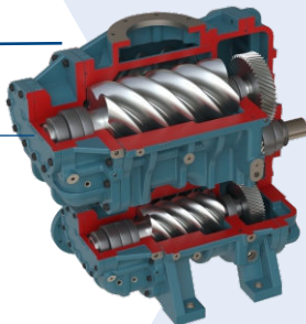
"SKY" SERIES AIR END Maximum Output with Less Energy Usage
